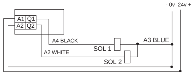
Siemens Wiring Schematic with Dual Output to Interface to Safety Exhaust Valve
