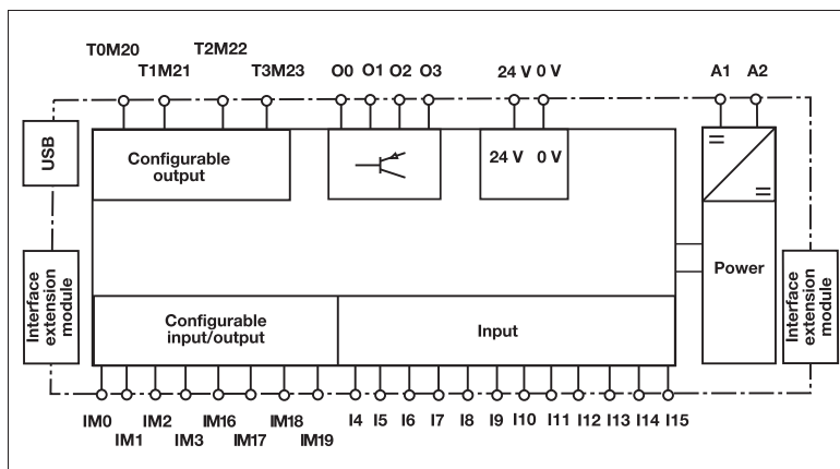
Block diagram
